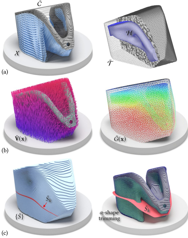
Fig. 8. An illustration of support generation: (a) a set of sample points \mathcal{X} for indicating the region of support and the tetrahedral mesh \tilde{\mathcal{T}} generated in the convex-hull \hat{C} = C(\mathcal{X} \cup \mathcal{H}) , (b) a new vector-field \tilde{\mathbf{V}}(\mathbf{x}) and the corresponding scalar-field \tilde{G}(\mathbf{x}) computed in \tilde{\mathcal{T}} by extrapolating \mathbf{V}(\mathbf{x}) , and (c) extracting iso-surfaces of \tilde{G}(\mathbf{x}) as \{\tilde{S}_k\} and trimming them by the \alpha -shape of \mathcal{X} .
